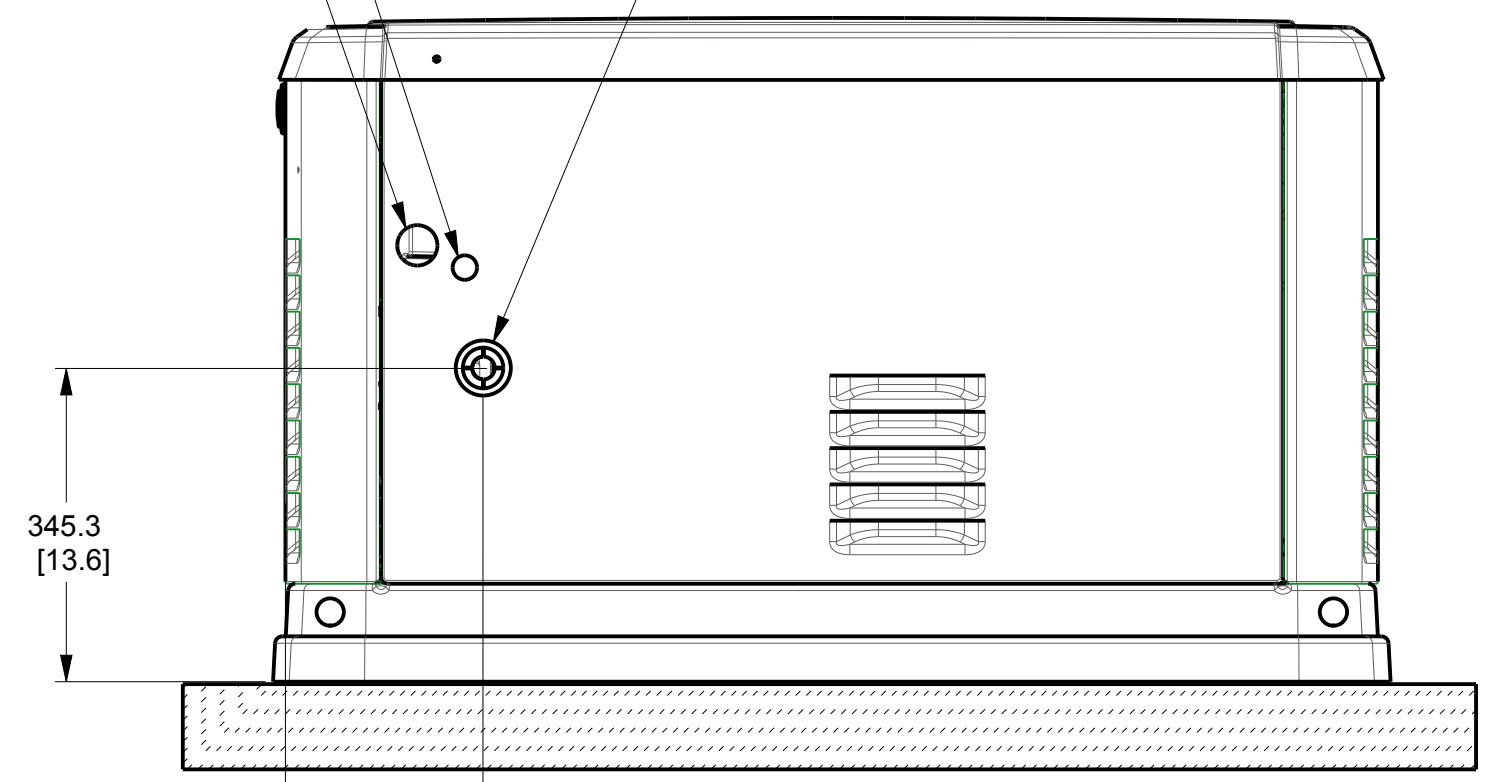
REAR VIEW
